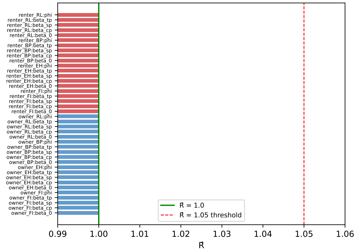
Gelman-Rubin R
