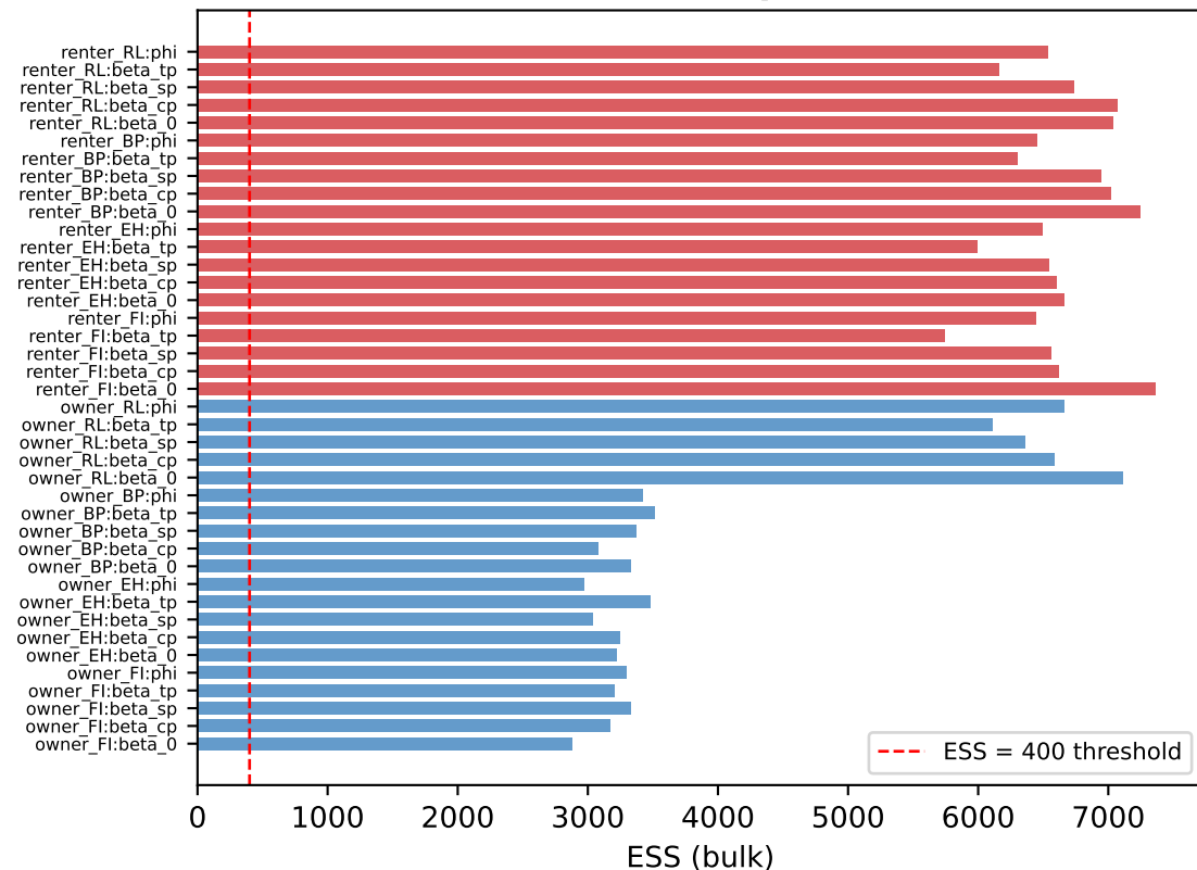
Effective Sample Size
