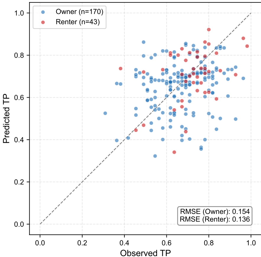
Goodness of Fit: Observed vs Predicted TP
