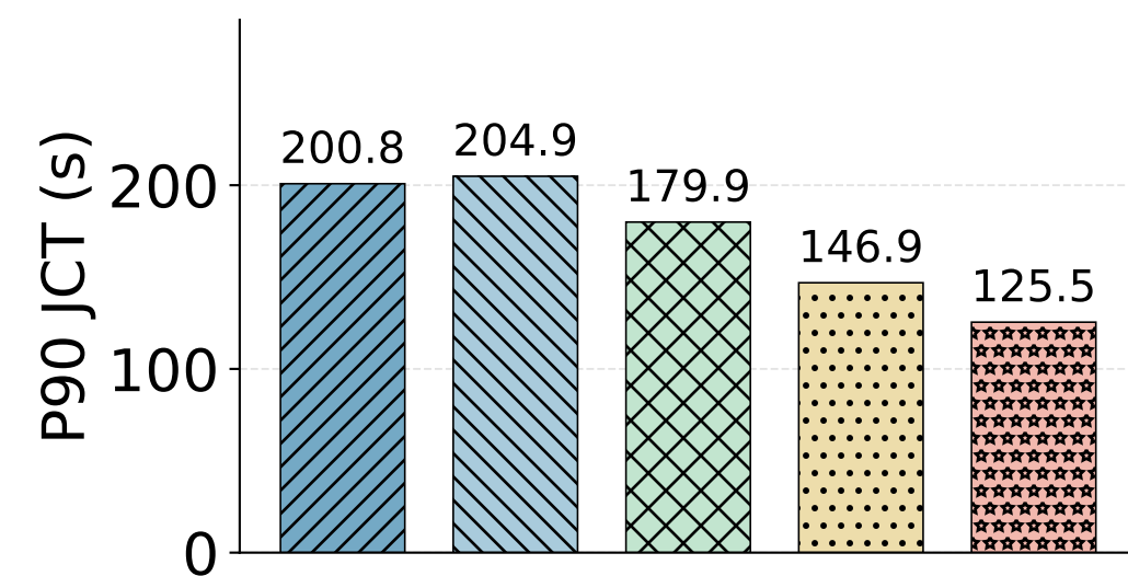
Qwen3-14B A100(80G)-TP1
