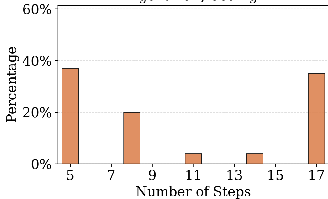
AgentFlow, Coding
