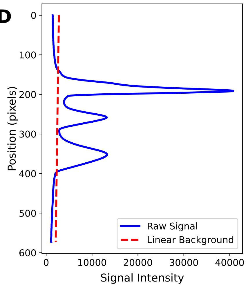
D Raw Signal vs Linear Background
