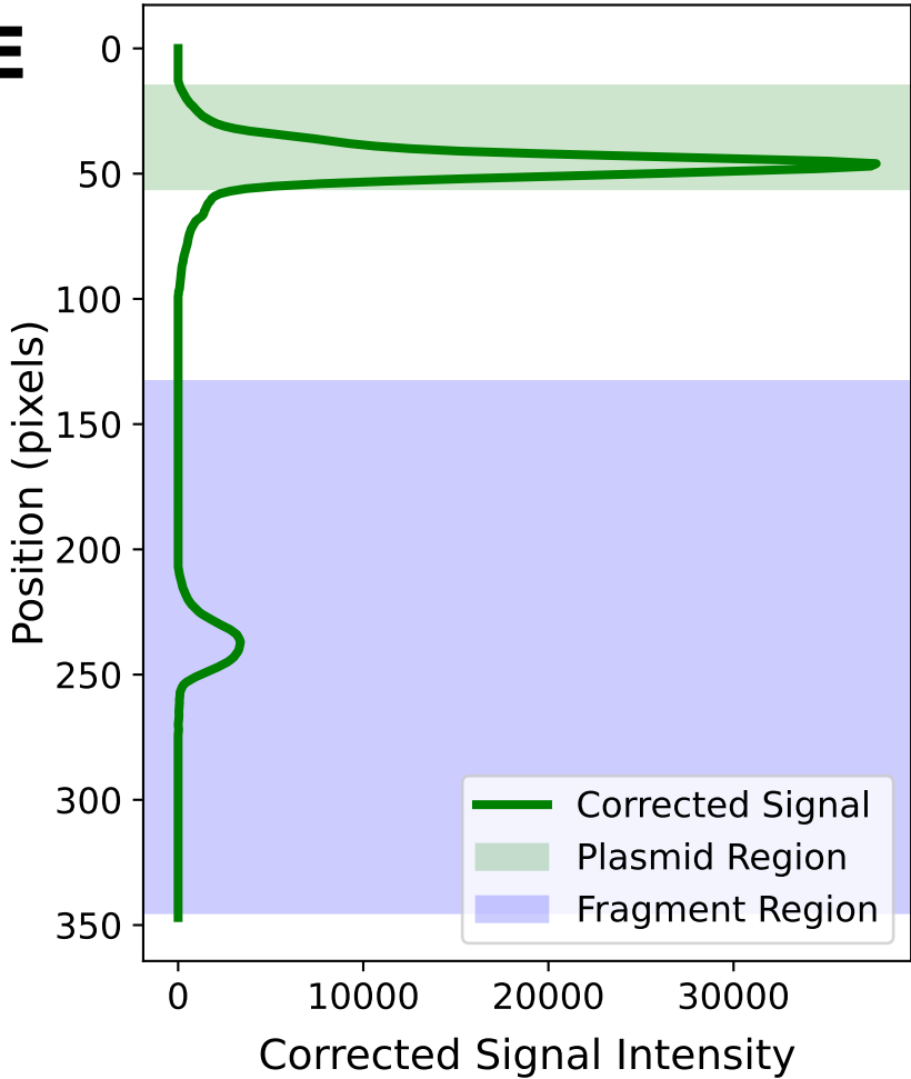
Background-Corrected Signal Plasmid: 432537, Fragment: 75331 Ratio: 0.15
