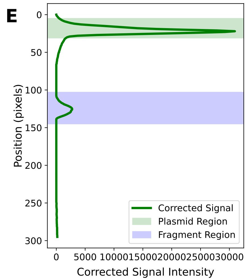
Background-Corrected Signal Plasmid: 264716, Fragment: 41335 Fraction: 0.14
