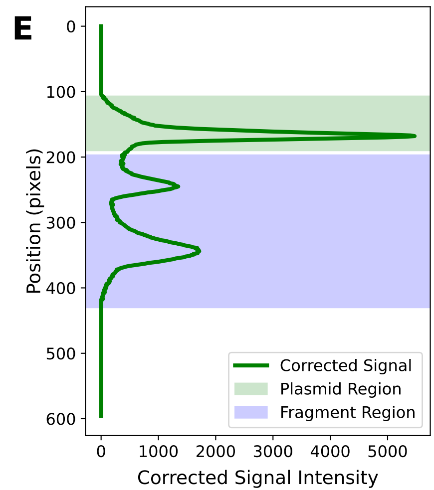
Background-Corrected Signal Plasmid: 101721, Fragment: 130595 Ratio: 0.56
