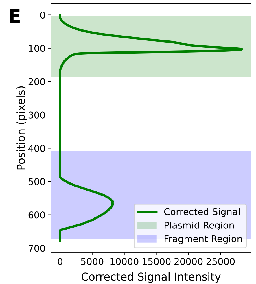
Background-Corrected Signal Plasmid: 1127270, Fragment: 779369 Ratio: 0.41
