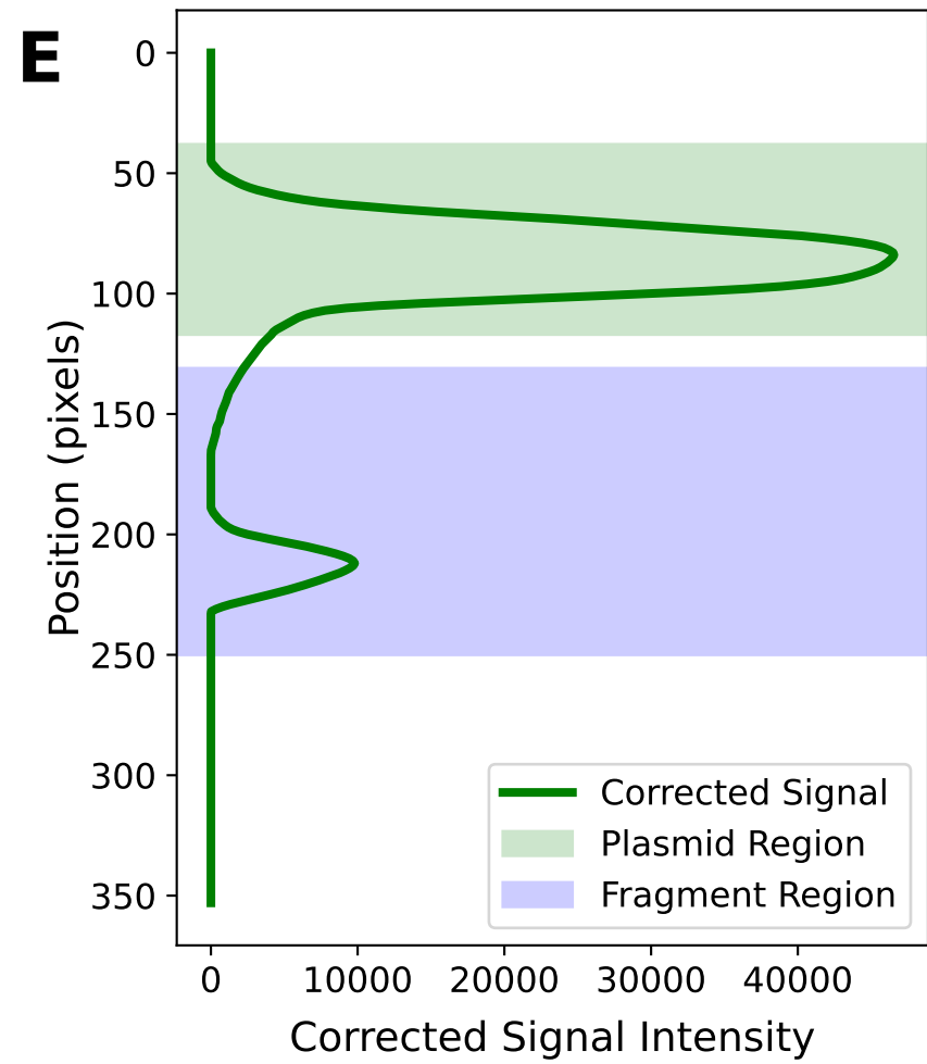
Background-Corrected Signal Plasmid: 1576801, Fragment: 232915 Ratio: 0.13
