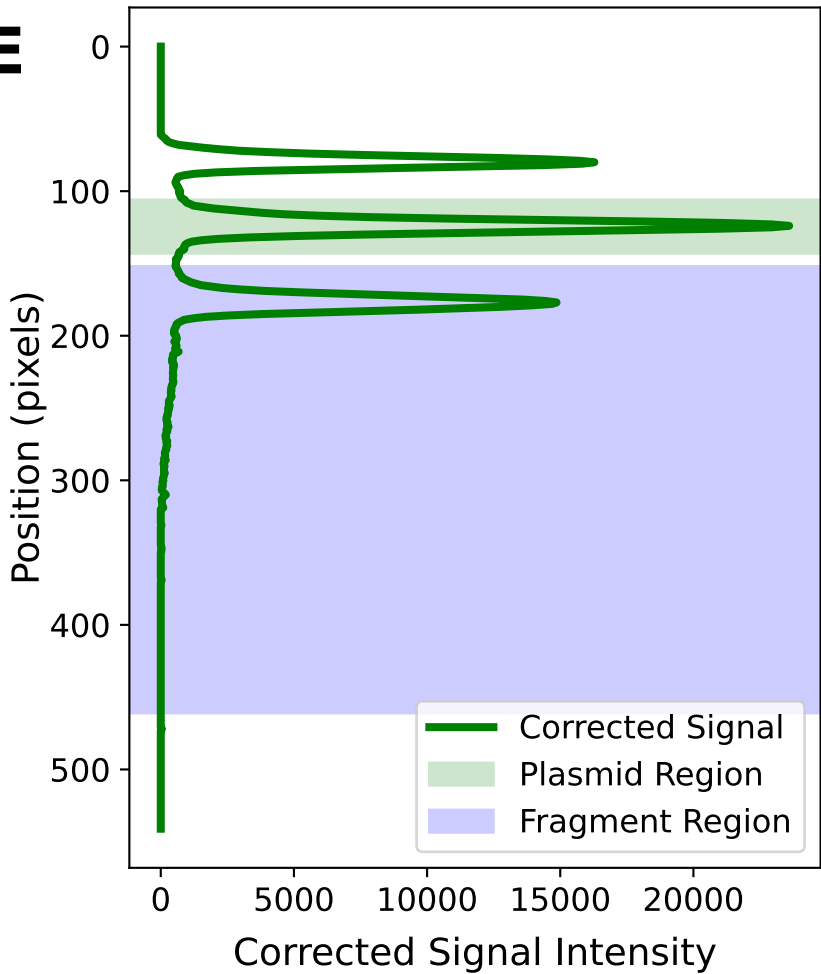
Background-Corrected Signal Plasmid: 262127, Fragment: 235564 Ratio: 0.47
