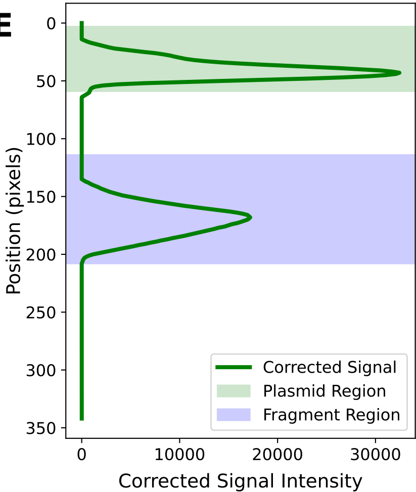
Background-Corrected Signal Plasmid: 554505, Fragment: 560212 Fraction: 0.50
