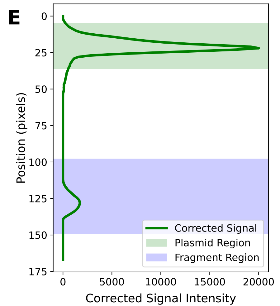
Background-Corrected Signal Plasmid: 173407, Fragment: 23907 Ratio: 0.12
