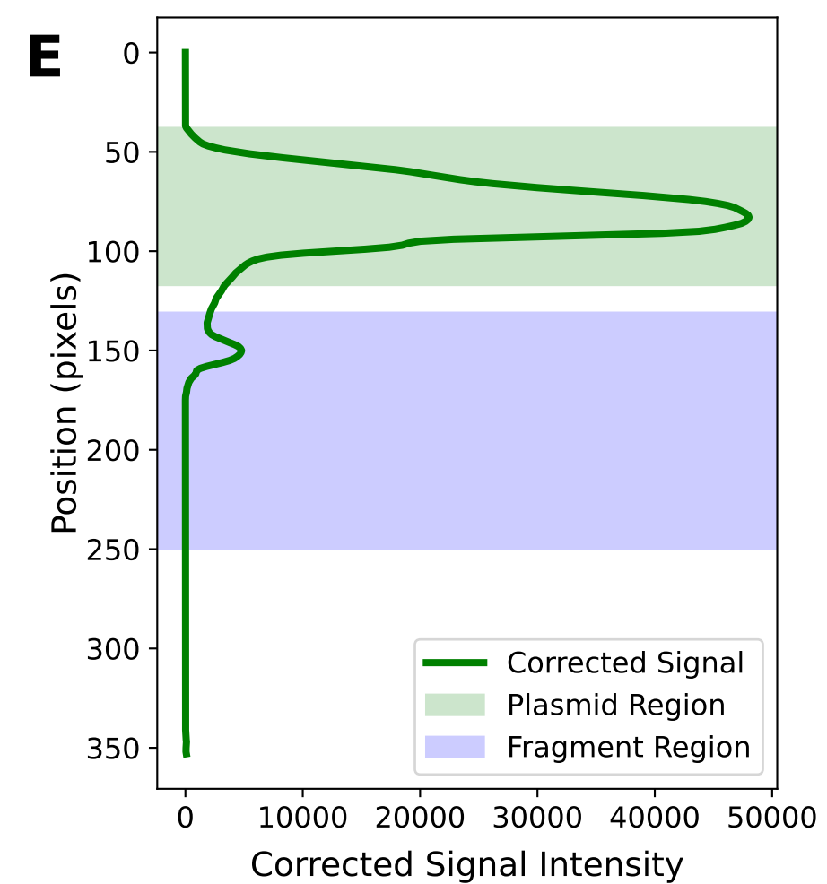
Background-Corrected Signal Plasmid: 1624722, Fragment: 90324 Ratio: 0.05
