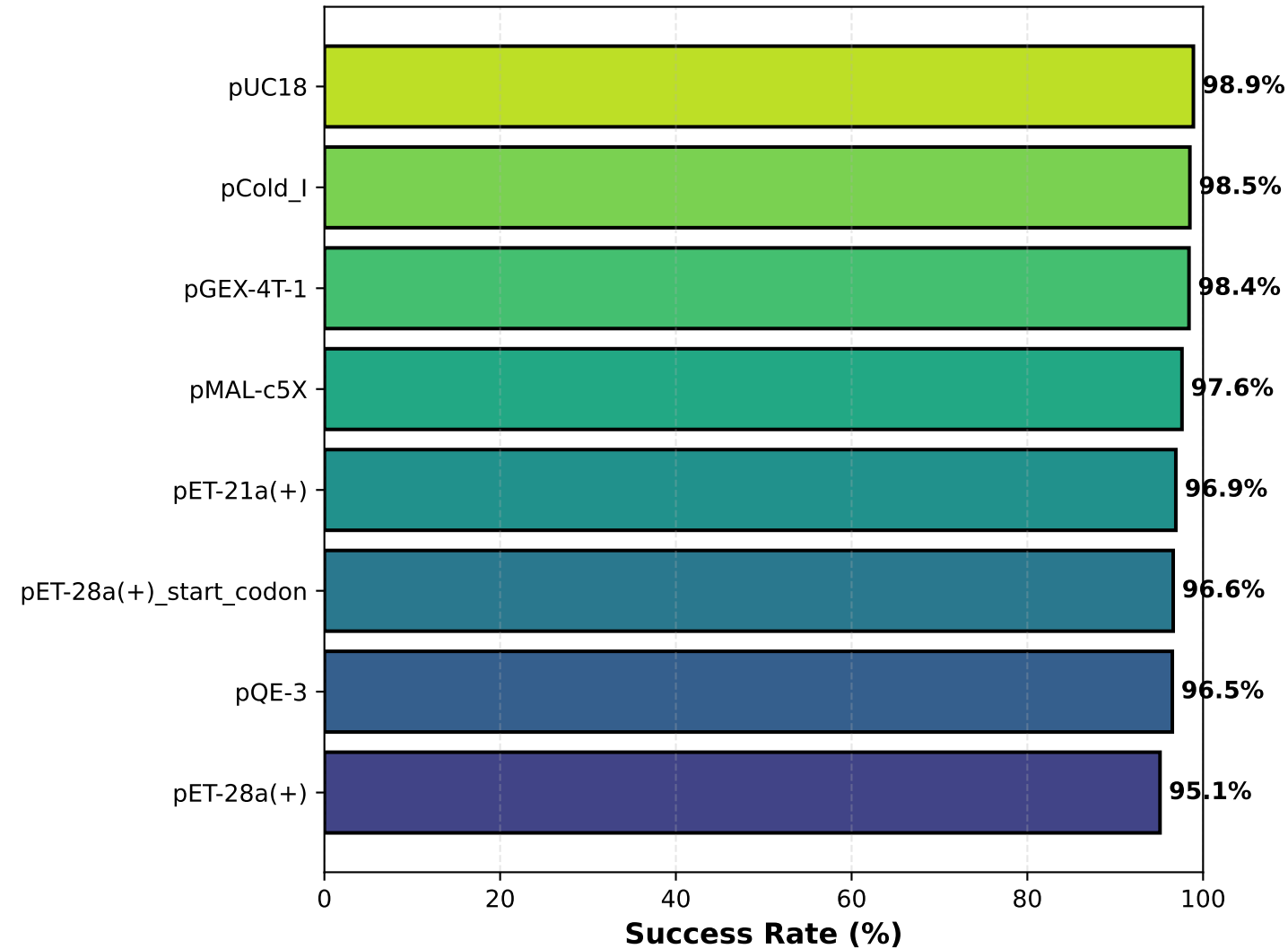
Success Rate at 60 AA by Plasmid
