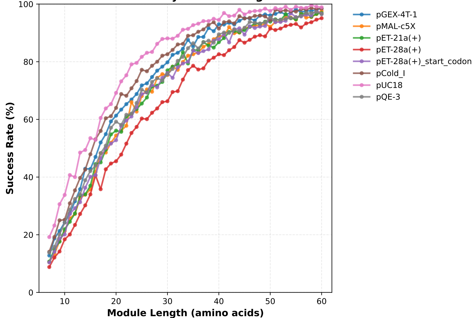
HURDLER Success Rate by Module Length and Plasmid
