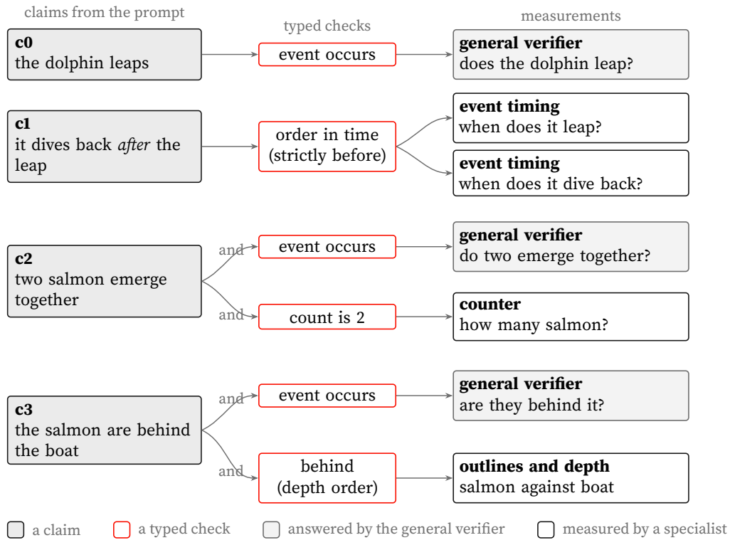
Figure 12: One prompt’s plan as a graph. Each claim the prompt makes becomes one or more typed checks, and each check names the measurements that would settle it. A claim can carry more than one check—a numeral adds a count beside the occurrence judgement, a spatial preposition adds a depth-ordered relation—and a single check can consume more than one measurement, as an ordering does. Occurrence and existence go to the general verifier reading the frames; quantities, timings, outlines and depths come from specialists. Illustrative: the plan is written in the report’s measurement vocabulary, and the claims are of the kinds the planner emits.
