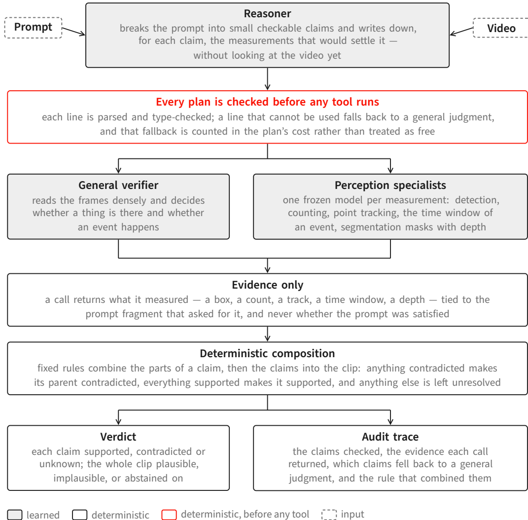
Figure 6: The critic. A reasoner turns the prompt into checkable claims and writes down the measurements that would settle each one; the plan is type-checked before any tool runs; a general verifier reading the frames densely decides whether things are present and events happen, while frozen specialists supply the quantities it cannot produce. Every call returns evidence only, and fixed rules — not a second model — turn that evidence into the verdict and the trace beside it. Shaded boxes are learned components; outlined boxes are deterministic.
