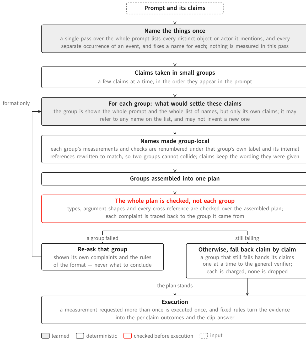
Figure 8: How a plan is constructed. One pass names everything the prompt talks about—the objects and actors, and each separate occurrence of an asserted event—and nothing else; the claims are then handled a few at a time against that fixed list, so that different parts of a long prompt refer to the same things. Each group’s identifiers are renumbered under its own label so groups cannot collide when assembled, and the assembled plan is checked as a whole, because what needs checking is mostly cross-reference. A group that fails is asked again with its own complaints and a restatement of the format, never with the answer; a group that still fails hands its claims to the general verifier one at a time, charged to the plan’s cost. Shaded boxes are learned components; outlined boxes are deterministic.
