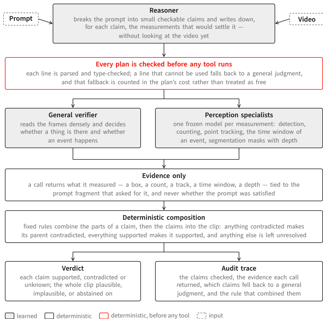
Figure 9: The critic. A reasoner turns the prompt into checkable claims and writes down the measurements that would settle each one; the plan is type-checked before any tool runs; a general verifier reading the frames densely decides whether things are present and events happen, while frozen specialists supply the quantities it cannot produce. Every call returns evidence only, and fixed rules — not a second model — turn that evidence into the verdict and the trace beside it. Shaded boxes are learned components; outlined boxes are deterministic.
