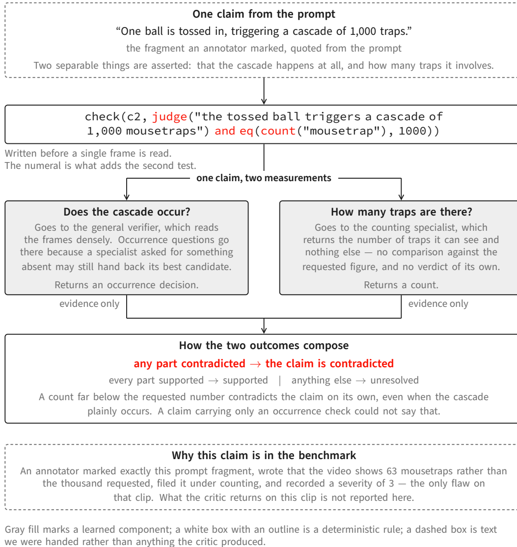
Figure 9: One claim, two measurements. A numeral in the claim adds a counting check beside the occurrence judgment, and the composition rule lets the count alone contradict the claim even when the cascade plainly happens. The prompt and the annotator’s record shown at the foot are real; what the critic returns on this clip is not reported here.
