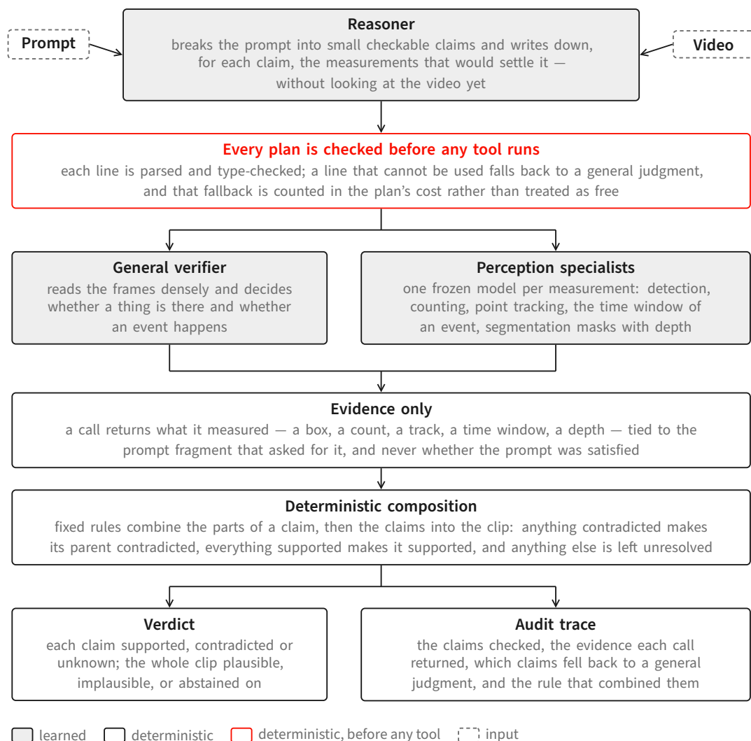
Figure 8: The critic. A reasoner turns the prompt into checkable claims and writes down the measurements that would settle each one; the plan is type-checked before any tool runs; a general verifier reading the frames densely decides whether things are present and events happen, while frozen specialists supply the quantities it cannot produce. Every call returns evidence only, and fixed rules — not a second model — turn that evidence into the verdict and the trace beside it. Shaded boxes are learned components; outlined boxes are deterministic.
