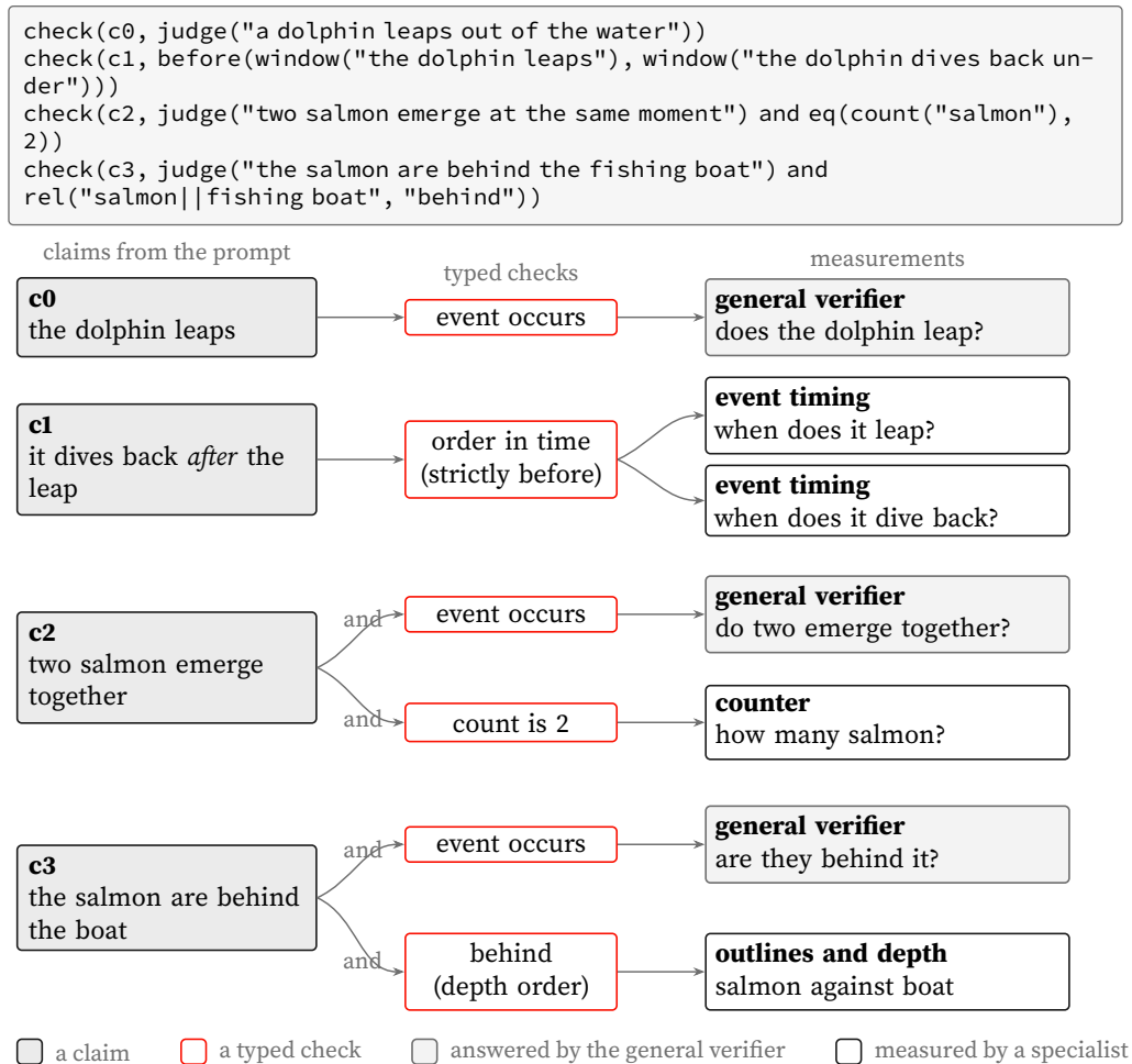
Figure 10: One prompt’s plan as a graph. Each claim the prompt makes becomes one or more typed checks, and each check names the measurements that would settle it. A claim can carry more than one check—a numeral adds a count beside the occurrence judgement, a spatial preposition adds a depth-ordered relation—and a single check can consume more than one measurement, as an ordering does. Occurrence and existence go to the general verifier reading the frames; quantities, timings, outlines and depths come from specialists. Illustrative: the plan is written in the report’s measurement vocabulary, and the claims are of the kinds the planner emits.
