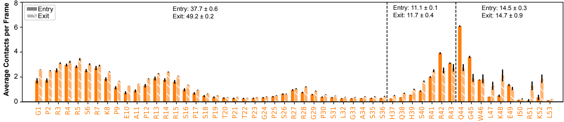
H3 Tail+Latch+αN CENP-A Core Average Contacts Per Frame
