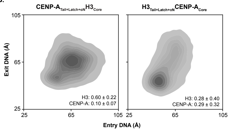
CENP-A Tail+Latch+αN H3 Core Average Contacts Per Frame
