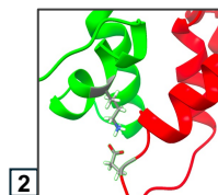
ARG59-GLU55
