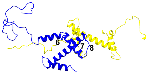
GLU105-ARG88
