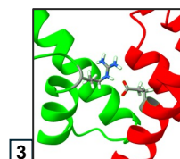
ARG92-GLU73
