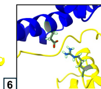
GLU105-ARG88
