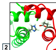
HIE75-GLU90
