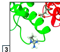
LYS69-GLU55
