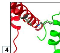
LYS91-GLU68
