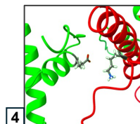
GLU72-LYS43
