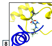
ARG134-GLU91
