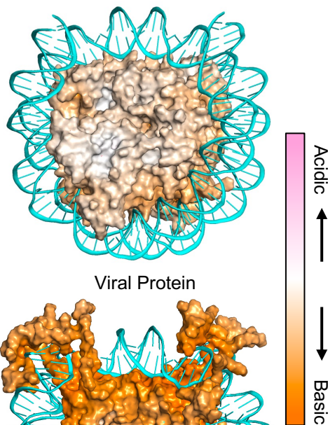
c) Surface Electrostatic Potential
