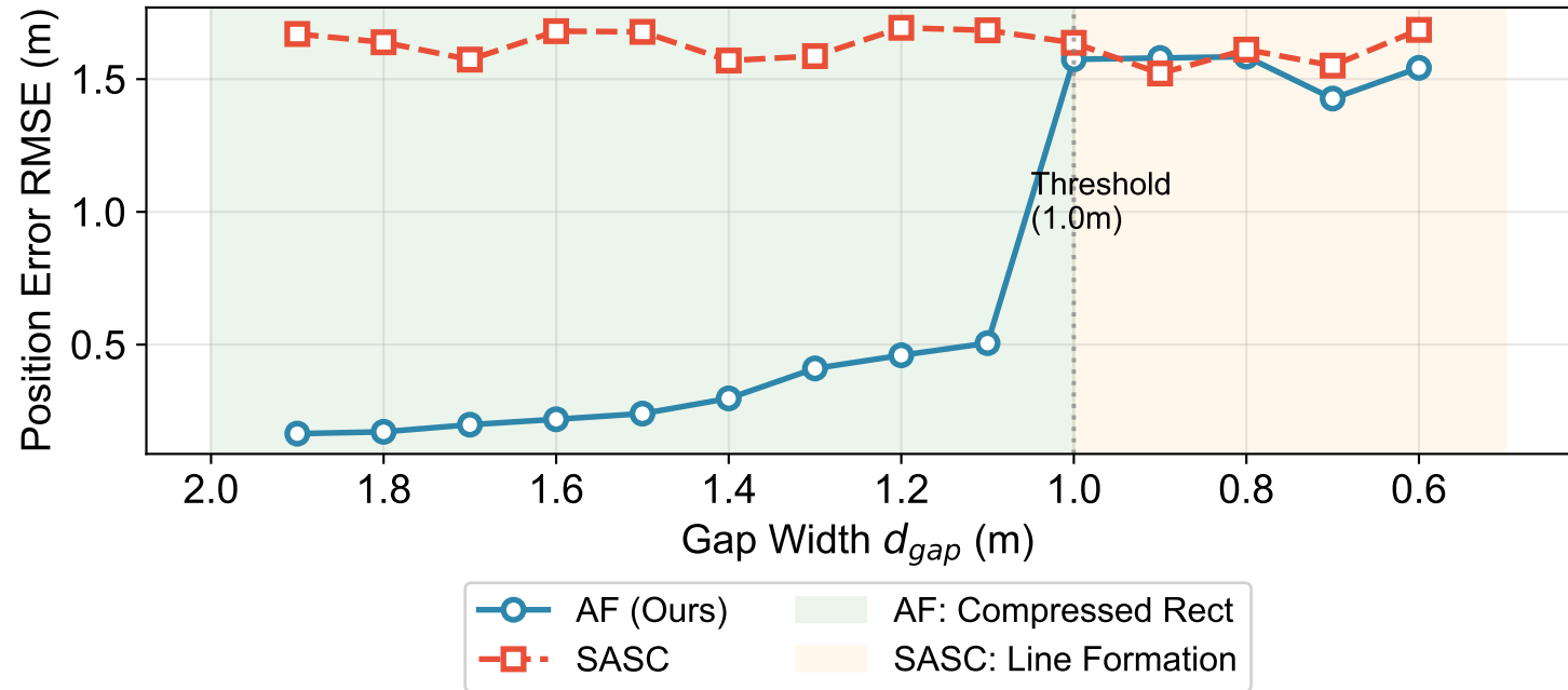
Formation Position Error vs. Narrow Gate Width
