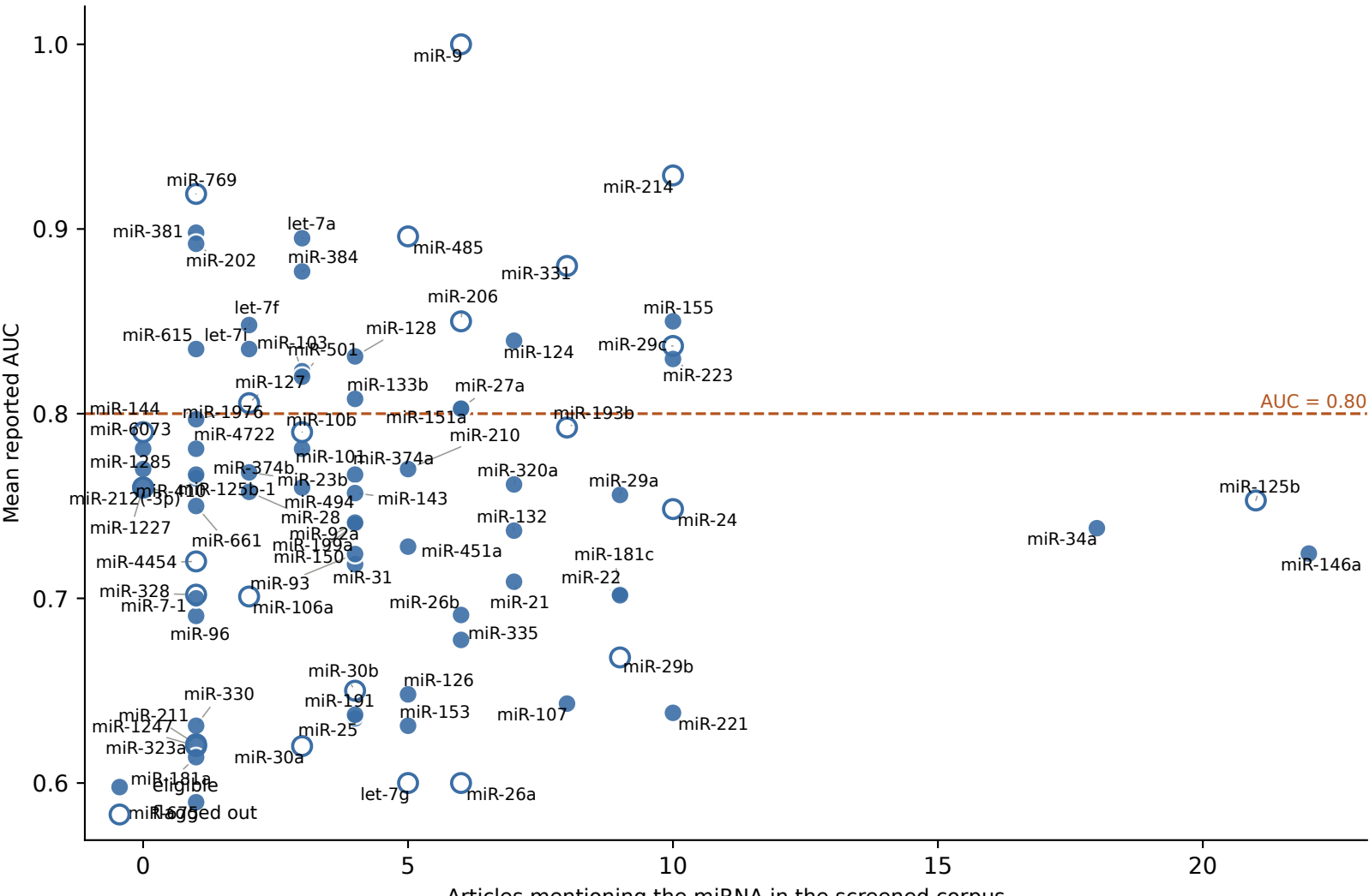
Literature attention does not track diagnostic performance
