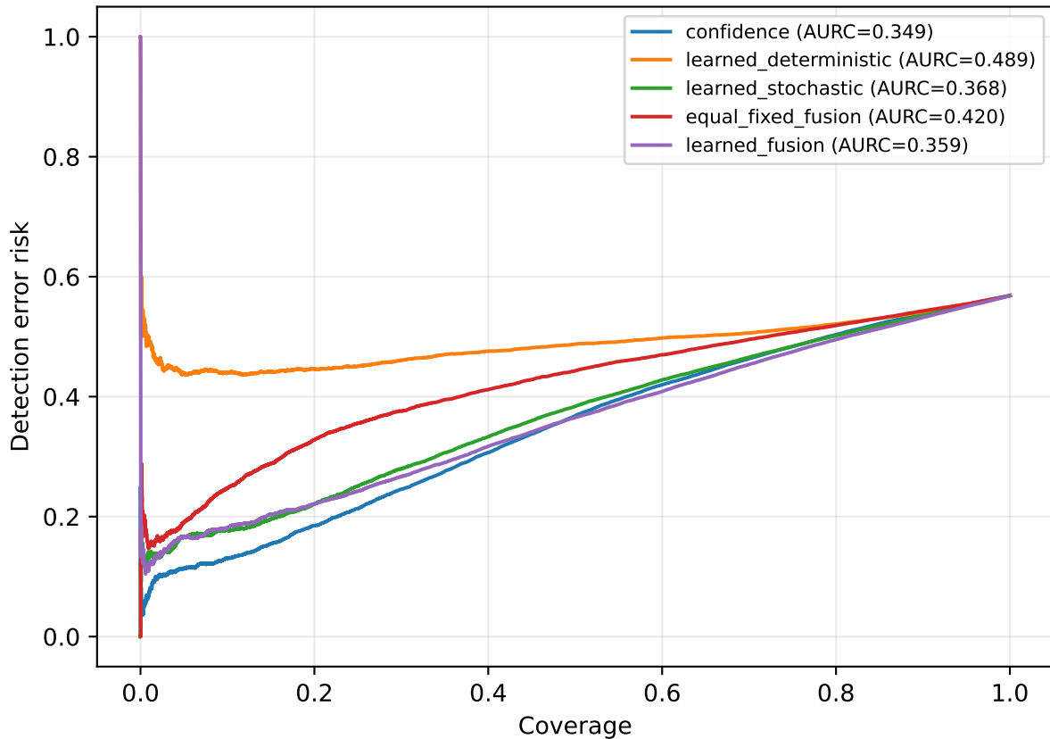
RQ2 risk-coverage comparison
