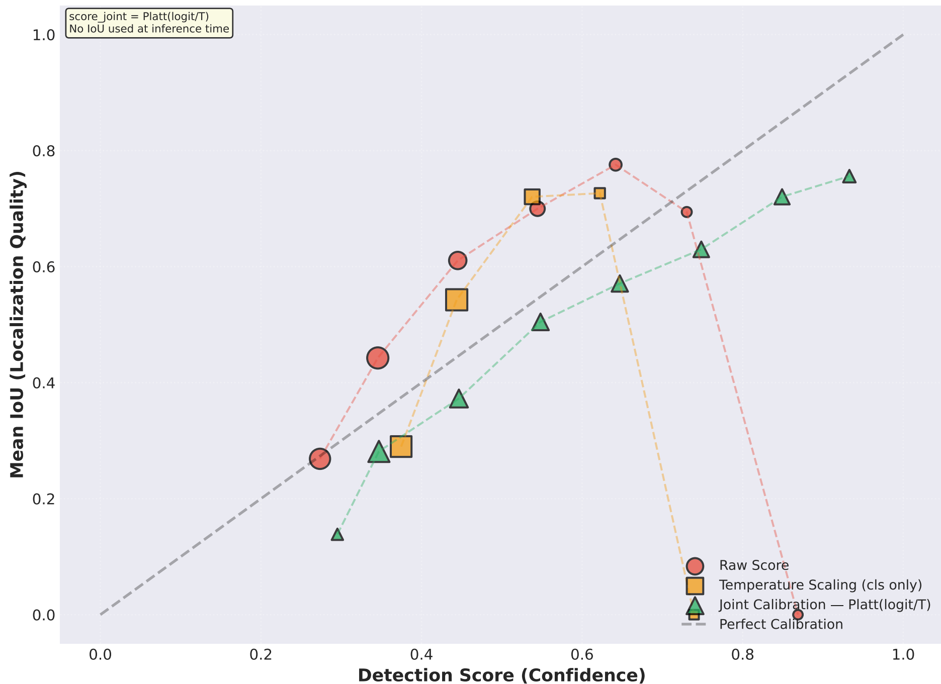
Figure RQ8.1. Reliability of Detection Scores vs Geometric Quality Evaluated on held-out test split (test split (30%, held-out))
