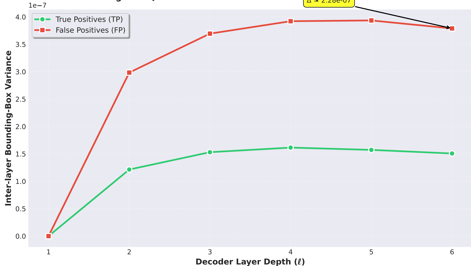
Figure RQ6.1: Decoder Variance Across Depth for TP vs FP
