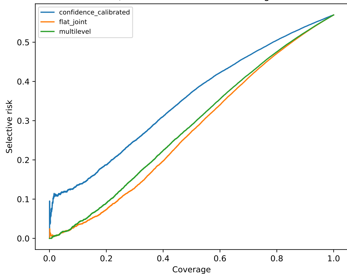
RQ4 shifted-domain risk--coverage
