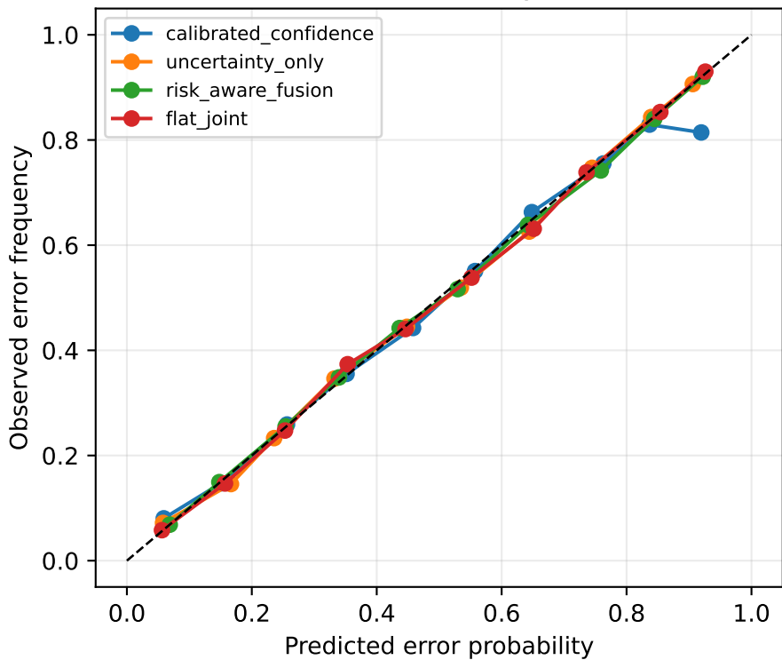
RQ5 reliability
