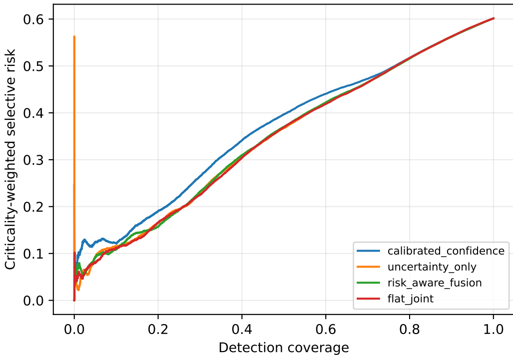
RQ5 weighted risk-coverage
