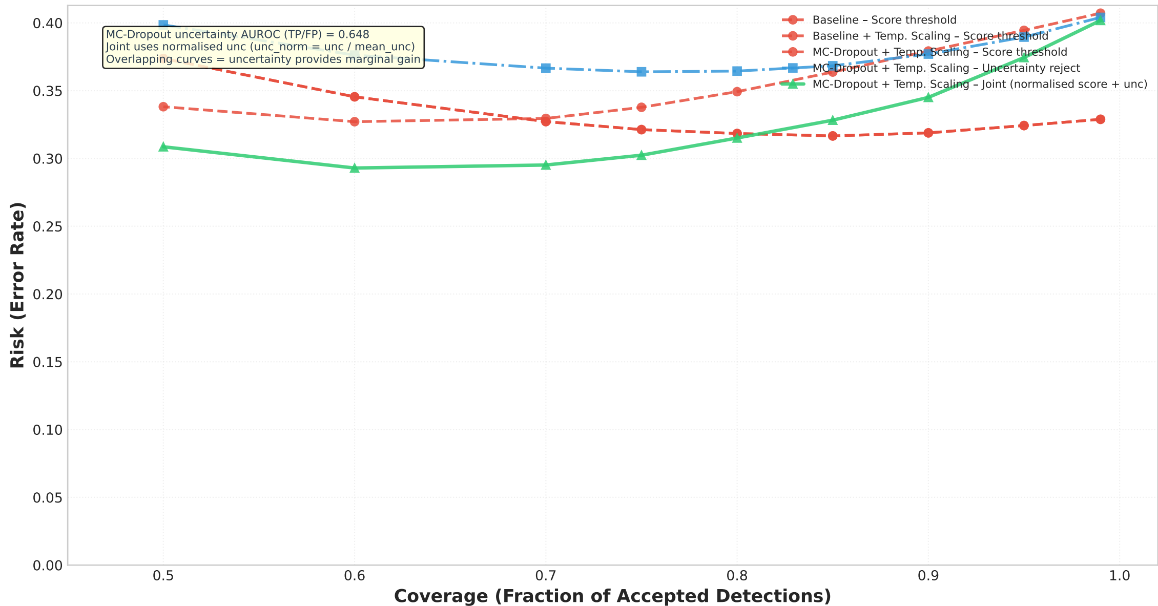
Figure RQ10.1: Selective Detection Risk-Coverage Trade-off Real data: score threshold, uncertainty reject, and joint (normalised) — MC-Dropout + Temp. Scaling
