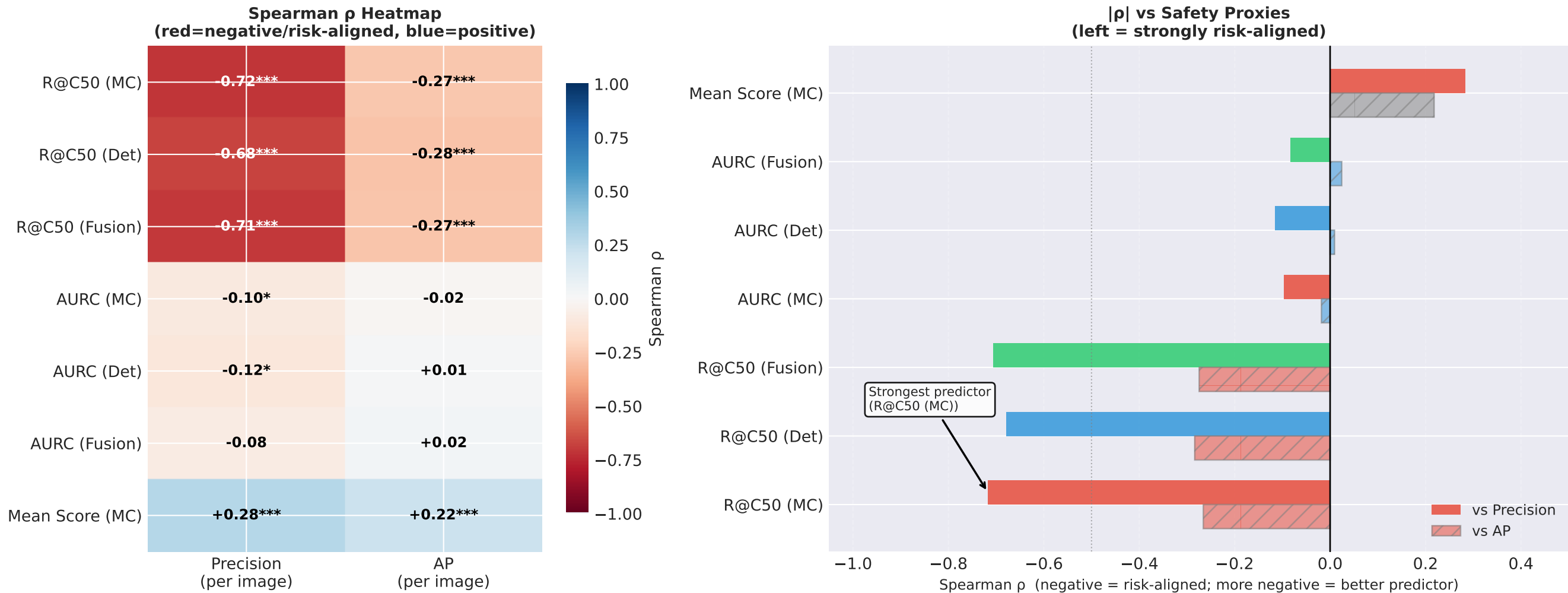
Figure RQ7.4. Spearman \rho between risk-aware metrics and per-image deployment safety. R@C50 shows the strongest alignment with operational safety (precision proxy): \rho \approx -0.72 (MC), -0.68 (Det), -0.71 (Fusion). Per-image AURC has near-zero correlation with AP ( |\rho| < 0.03 ), limited by small per-image sample sizes. mAP (mean score proxy) correlates at \rho \approx +0.28 , substantially weaker than R@C50. *** p < 0.001 , ** p < 0.01 , * p < 0.05 .
