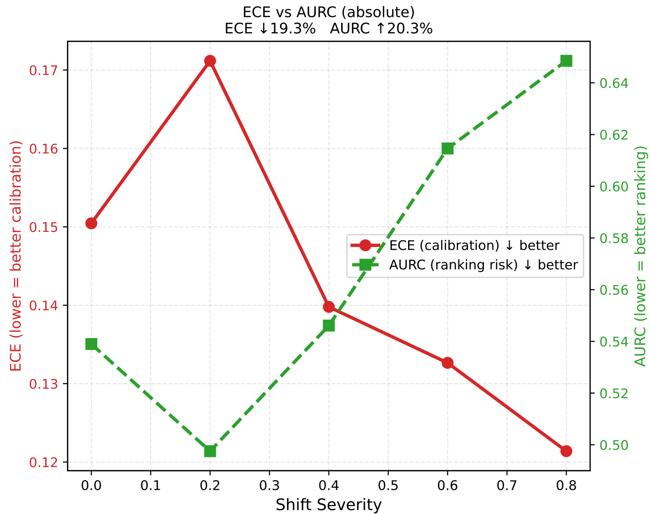
Figure RQ9.1. Metric Behavior under Distribution Shift
