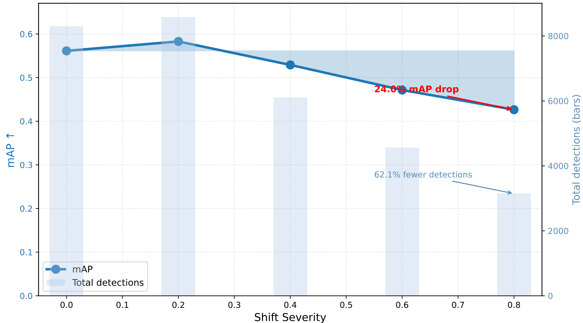
Figure RQ9.2. Accuracy Collapse and Detection Suppression under Distribution Shift
