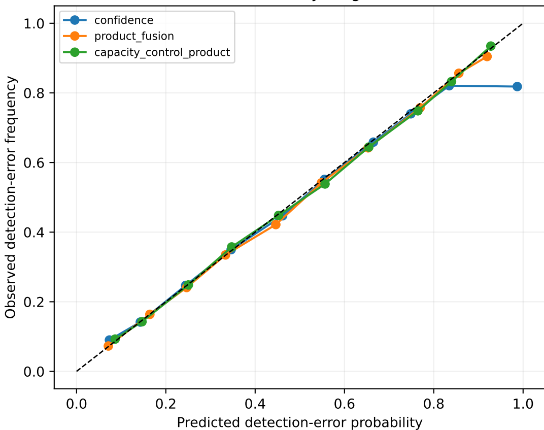
RQ3 reliability diagram
