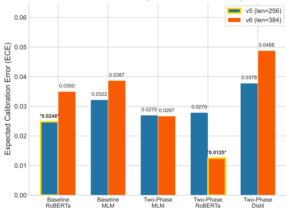
Model Calibration (lower is better, * = best)
