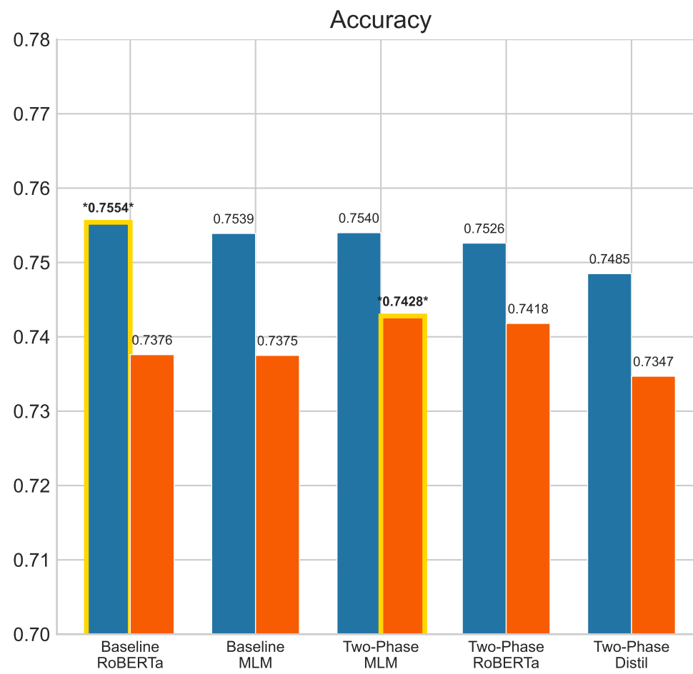
Model Performance: v5 vs v6 (* = best in version)
