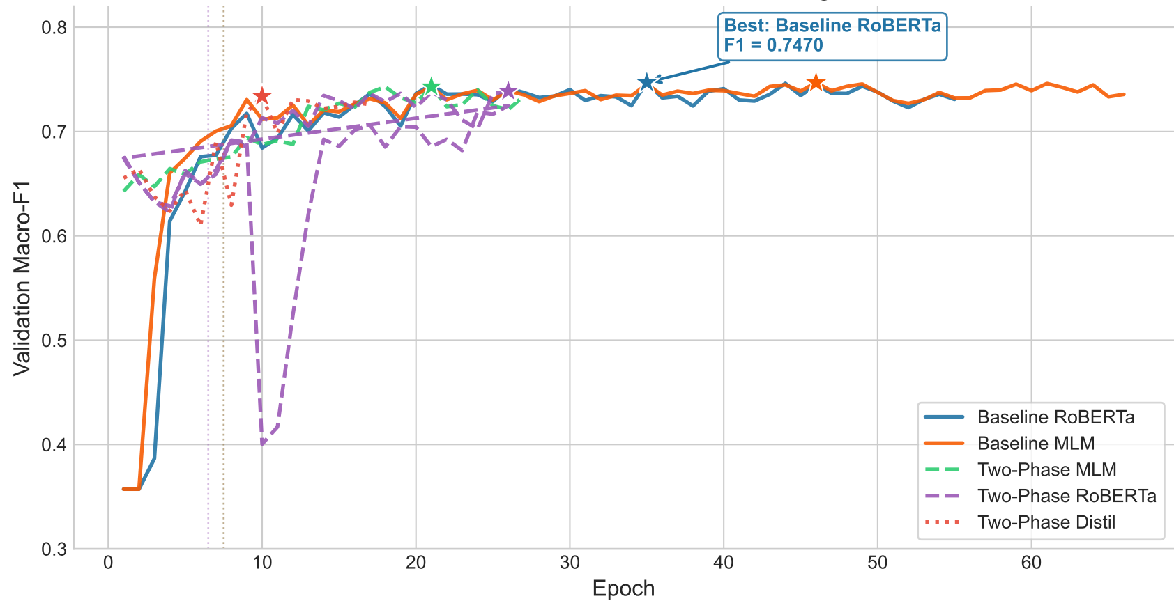
Validation Macro-F1 Across Training
