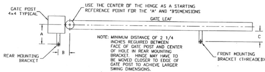
INWARD SWING MOUNTING OPTION
