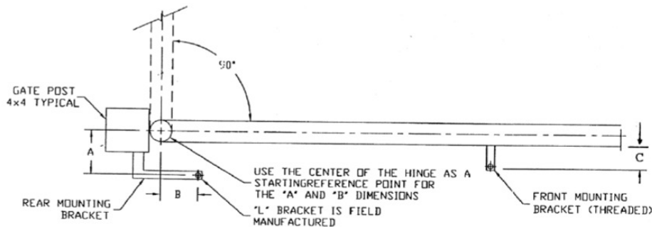
OUTWARD SWING MOUNTING OPTION
