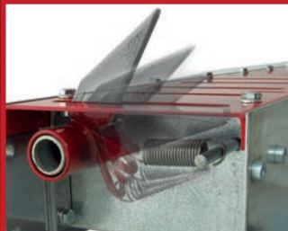
Flush Mount available with weighted or spring loaded spikes
