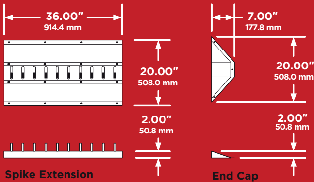
Surface Mount Spike Assembly
