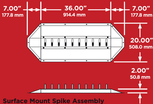
Surface Mount Spike Assembly
