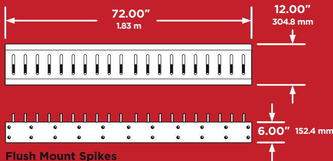
Flush Mount Spikes
