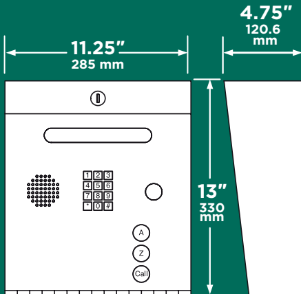
1834 Surface Mount
