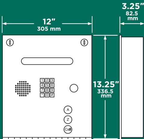
1834 Flush Mount
