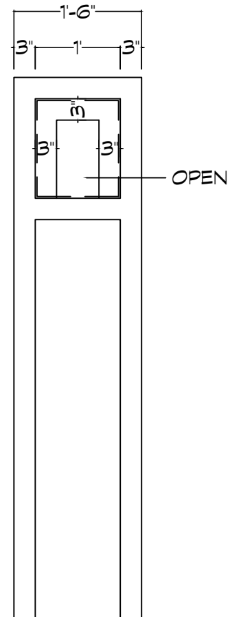
FRONT VIEW ELEVATION
