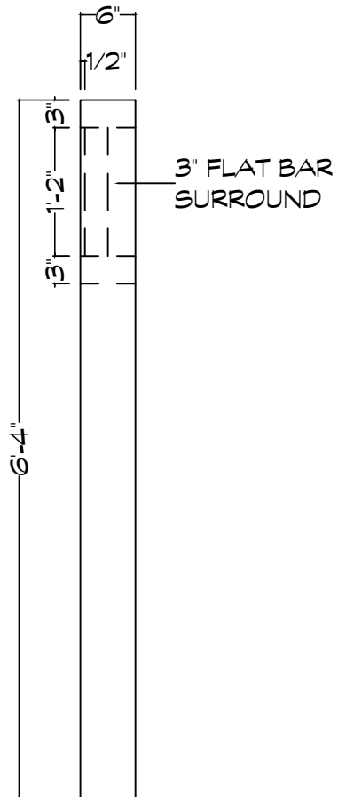
SIDE VIEW ELEVATION
