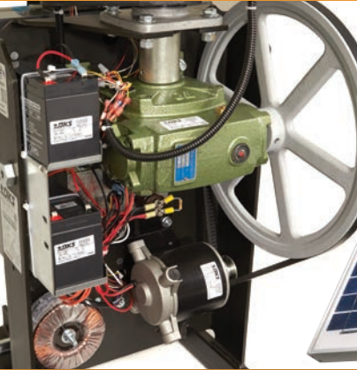
Heavy-duty gearbox and Quadra Drive DC motor
