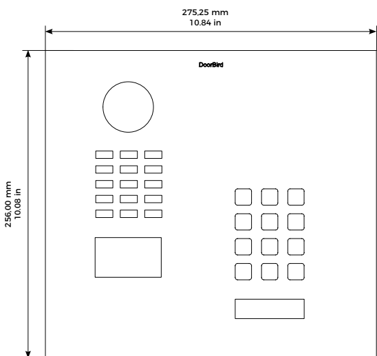
Frontpanel
