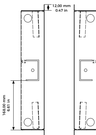
Flush-mounting housing (backbox)
