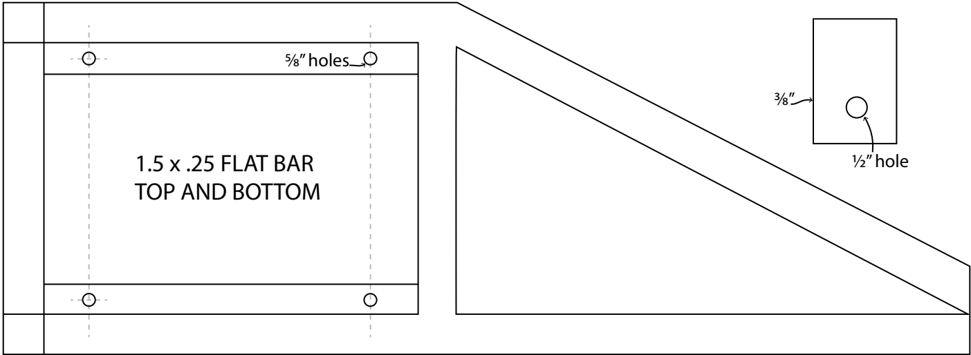
MOUNTING TAB
