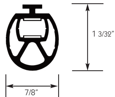
CPT-210 Extrusion
