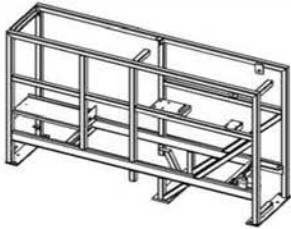
COMMERCIAL OPERATOR — 96" L x 23" W x 56" H
