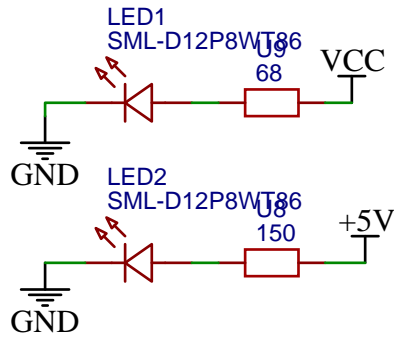
Voltage LEDs
