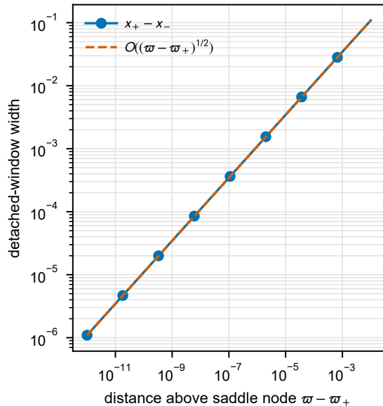
(b) Double-root conditioning
